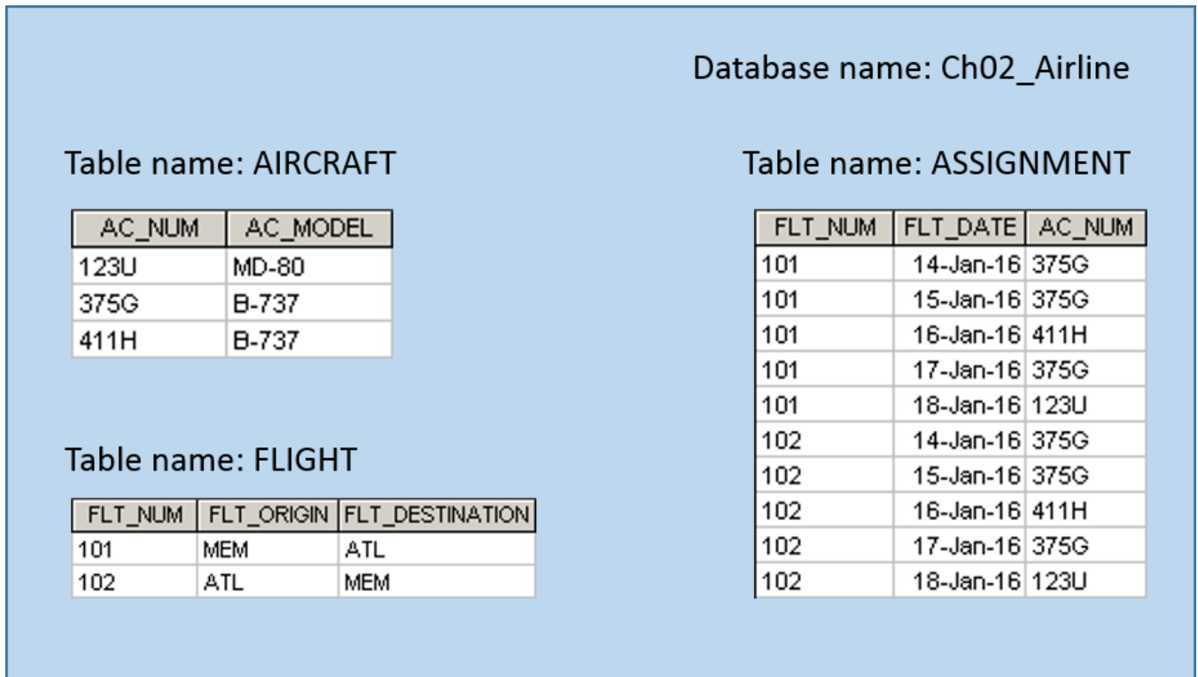
FIGURE P2.16c The Airline Database Tables
