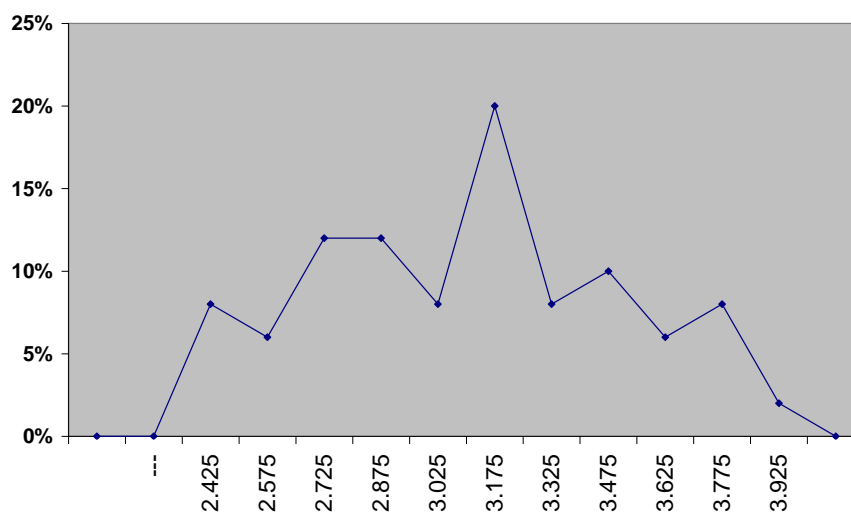
Percentage Polygon
