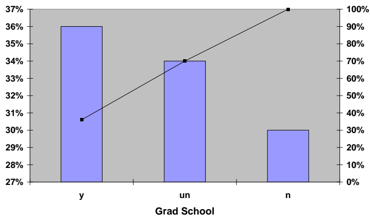
Pareto Diagram
