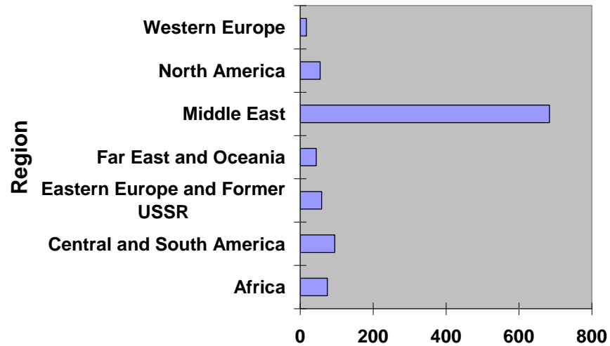
Bar Chart
