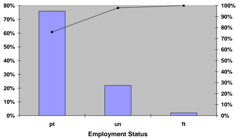
Pareto Diagram
