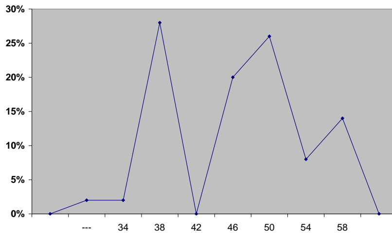
Percentage Polygon
