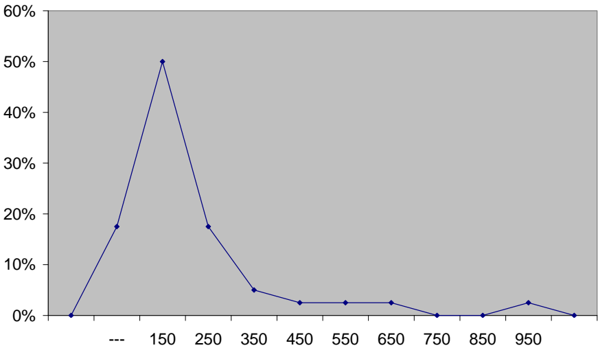
Percentage Polygon
