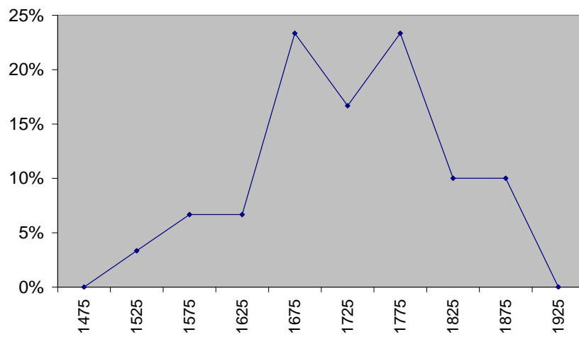
Percentage Polygon
